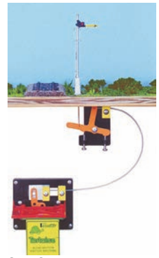
Gate/Semaphore Actuator Drive Mechanism Circuitron. 800-8100 w/Cable & Actuator Reg. Price: $14.95 Sale: $12.98
