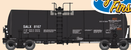
HO WalthersProto™ 40' Trinity 14,000-Gallon Molten Sulfur Tank Car pg 4
