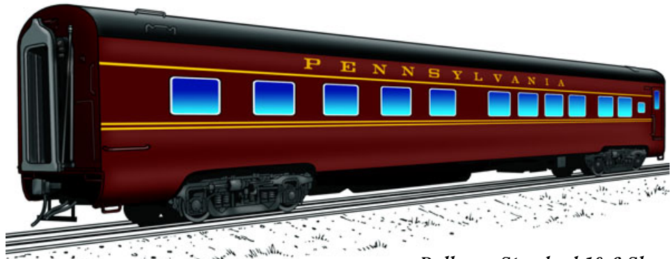
Pullman-Standard 10-6 Sleepers
