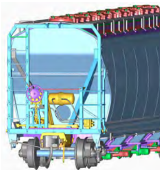
Revised end cage
