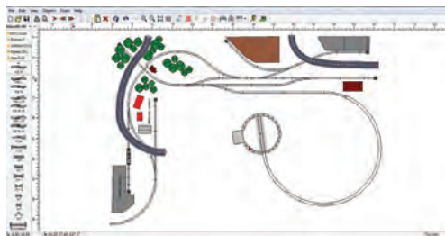
Software Interface
