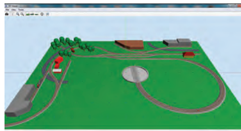
3D Viewer
