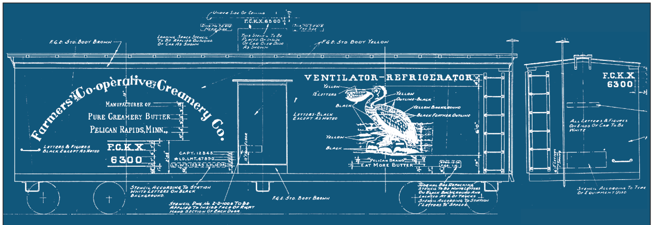
Pelican Brand 40' Wood Reefer Blueprint
